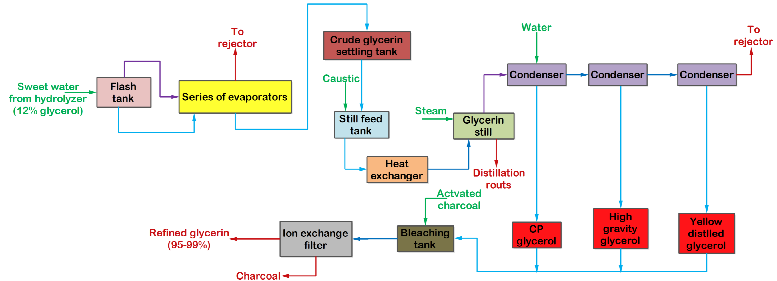
Figure: Manufacture of glycerol from sweet water
